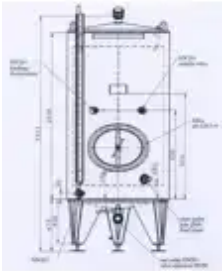
5.100 liters Storage tanks outside marbled for wine, water, fruit juice, schnapps with cooling jacket
